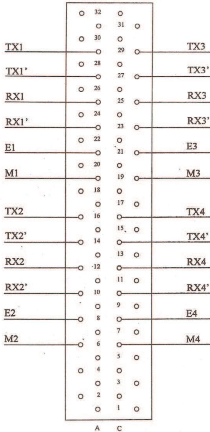
PIN DETAILS ON WIRE WRAPPABLE CONNECTOR FOR VOICE & G703 DATA INTERFACE
